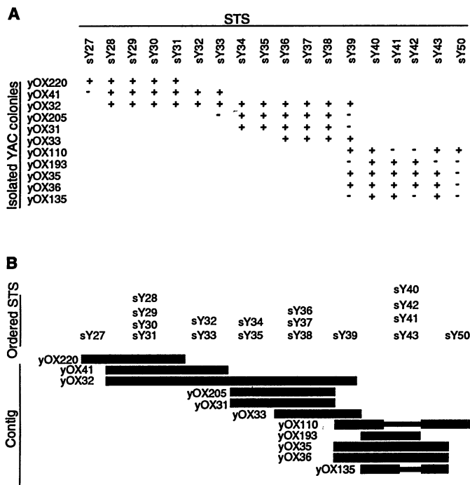
Fig. 1. Assembly of YAC contigs and ordering of STS's by STS content mapping. (A) Results of testing 11 Y-derived YAC's for the presence or absence of 18 STSs. The STS's present (indicated by a plus sign) in each YAC were initially ascertained during screening of the YAC library; all were confirmed by repeating PCR assays on DNA's from single colonies. Some negative results from library screening (those indicated by a minus sign) were reproduced on single colonies; no attempt was made to reproduce most negative results from library screening (indicated by the absence of any symbol). (B) Inferred overlaps among YAC's and inferred order of STSs, that is, the most economical interpretation of the data in (A). STS's stacked in piles are not ordered with respect to each other. Each YAC is represented by a black bar whose length is proportional to the number of STS's spanned; the drawing is otherwise not to scale. Some of the data in (A) (that is, the absence of sY41 and sY42 in yOX110, the absence of sY42 in yOX135) is inconsistent with the most likely order of STS's on the Y chromosome. These inconsistent data may reflect deletions within the inserts of yOX110 and yOX135, as represented by narrowed black bars.
